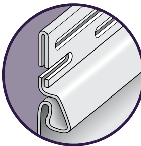
Extra-strong rolled over nail hem.
